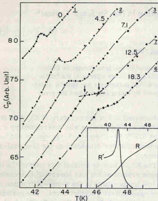
FIG. 1. Temperature dependence of the relative C_p at different pressures for \text{Nb}_3\text{Sn} single crystal. The inset shows the anomalies of resistance R and resistance slope R' at the T_L and atmospheric pressure.
