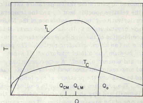
FIG. 3. Schematic variations of T_L and T_C with Q for \text{Nb}_3\text{Sn} (after Ref. 12).
