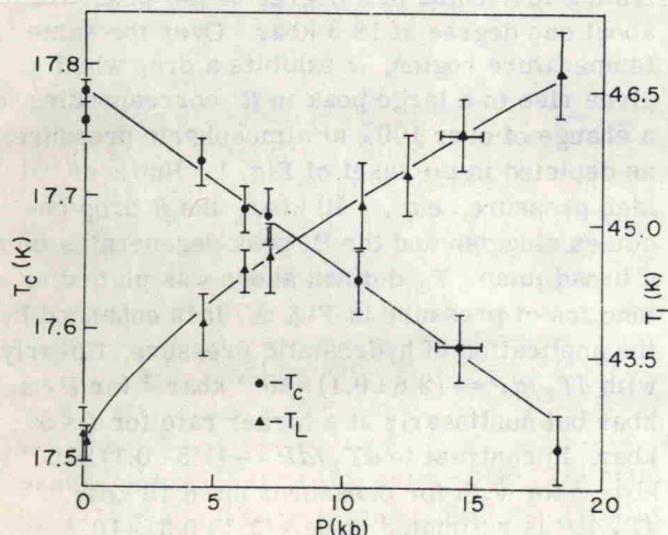
FIG. 2. Pressure dependence of T_L and T_C of \text{Nb}_3\text{Sn} single crystal.
